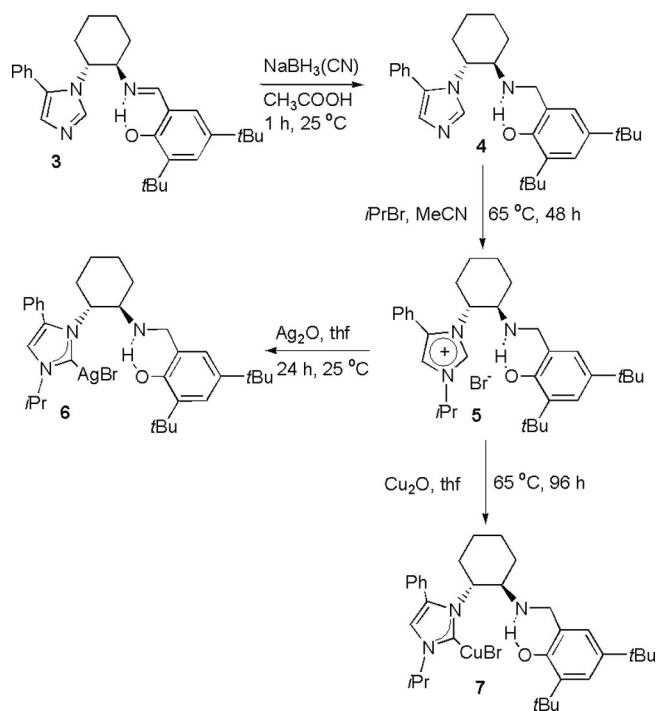
Scheme 2. Synthesis of NHC–phenolamine precursors and complexes 4–7 .
