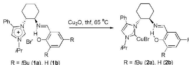
Scheme 1. Synthesis of Cu I NHC complexes derived from 1a and 1b .
