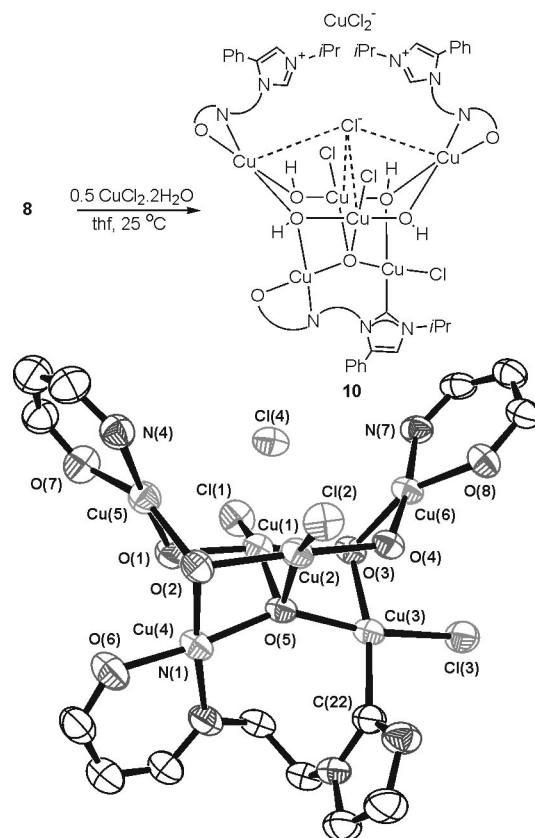
Figure 4. Synthesis and molecular structure of 10 . Hydrogen atoms, aryl, cyclohexyl, i Pr, t Bu, imidazolium groups and anions have been removed for clarity. Displacement ellipsoids at 50% probability level.
