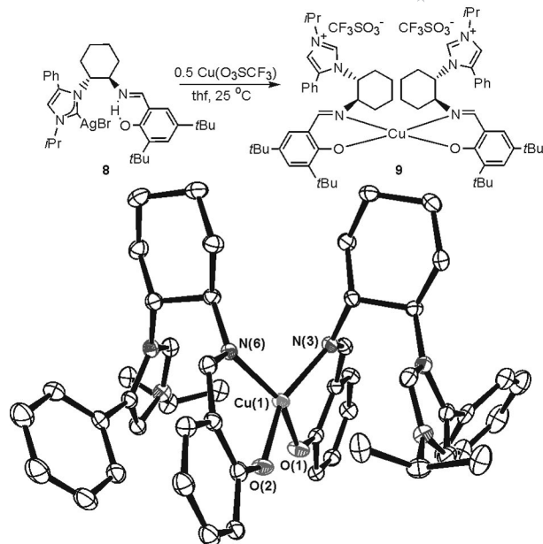
Figure 3. Synthesis and molecular structure of complex 9 . Hydrogen atoms, t Bu groups and anions have been removed for clarity. Displacement ellipsoids at 50% probability level.
