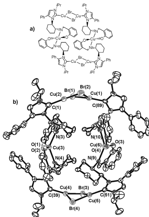
Figure 2. (a) Line drawing of 2b' . (b) The molecular structure of 2b' . Hydrogen atoms have been removed for clarity. Displacement ellipsoids at 50% probability level.
