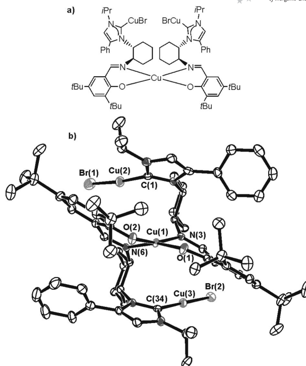
Figure 1. (a) Line drawing of 2a' . (b) Molecular structure of 2a' . Hydrogen atoms have been removed for clarity. Displacement ellipsoids at 50% probability level.
